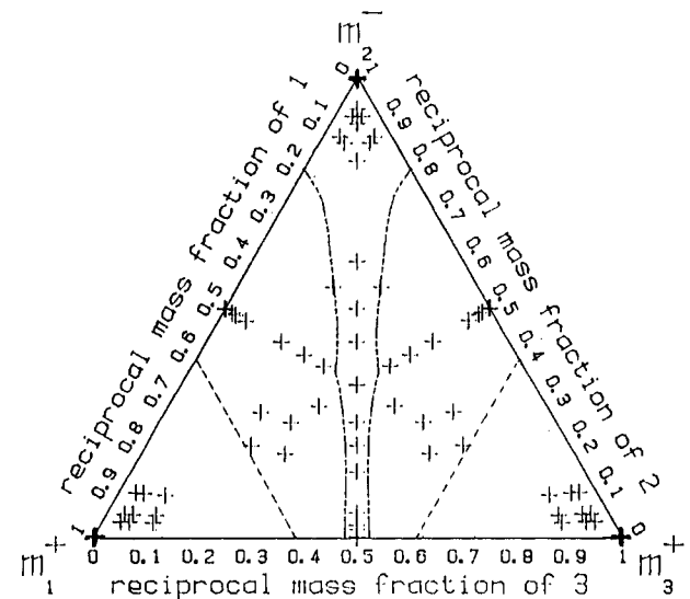
Figure 2. Reciprocal mass fraction ternary diagram for three-particle ions m_1^+m_2^-m_3^+ (or m_1^-m_2^+m_3^- ) showing all possible systems composed of e, \mu , p, d, and t as crosses. The two straight dashed lines are the critical binding curves predicted by a crude argument based on the critical dipole moment to bind a particle.
